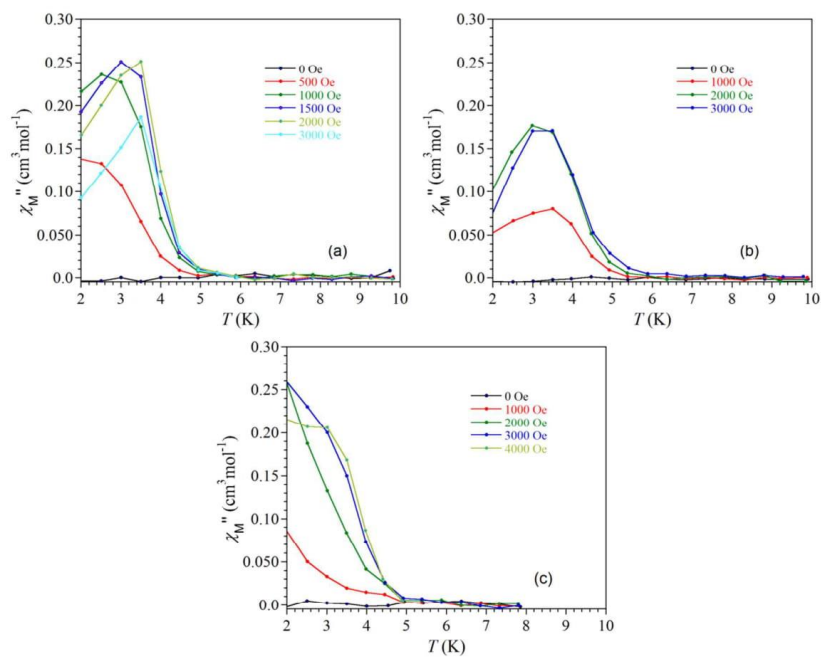
Figure S117. Temperature dependence of the out-of-phase ( \chi_M'' ) ac signals recorded at different dc fields with a 3 Oe ac field oscillating at 1000 Hz for (a) [\text{Fe}(\text{N}2_{\text{mes}})_2] (1), (b) [\text{Fe}(\text{N}2_{\text{Dipp}})_2] (2) and (c) [\text{Fe}(\text{HN}3_{\text{Dipp}})_2] \cdot \text{C}_2\text{H}_5\text{O} (3). The solid lines are guides for the eyes only.
