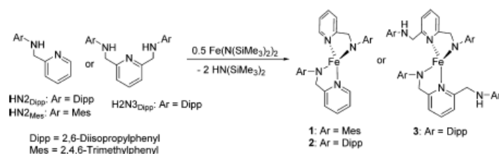
Scheme 1. Syntheses of Compounds 1–3
