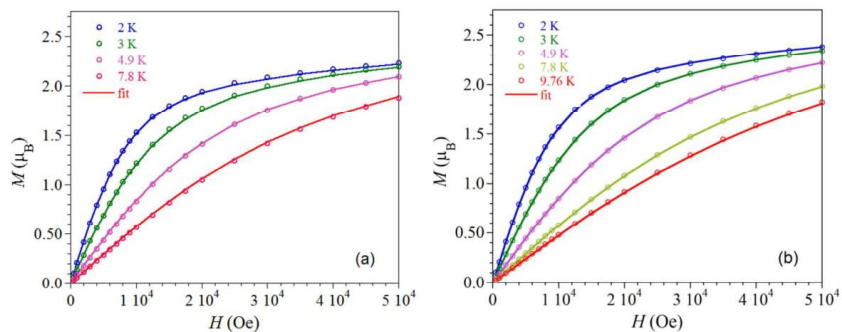
Figure S114. Field dependence of the magnetization ( M ) measured between 0 and 50000 Oe at temperatures ranging between 2 and 10 K for (a) [\text{Fe}(\text{N}2_{\text{Dipp}})_2] (2) and (b) [\text{Fe}(\text{HN}3_{\text{Dipp}})_2] (3) with the best fits obtained with the program PHI 10 in solid lines (see parameters in the text).
