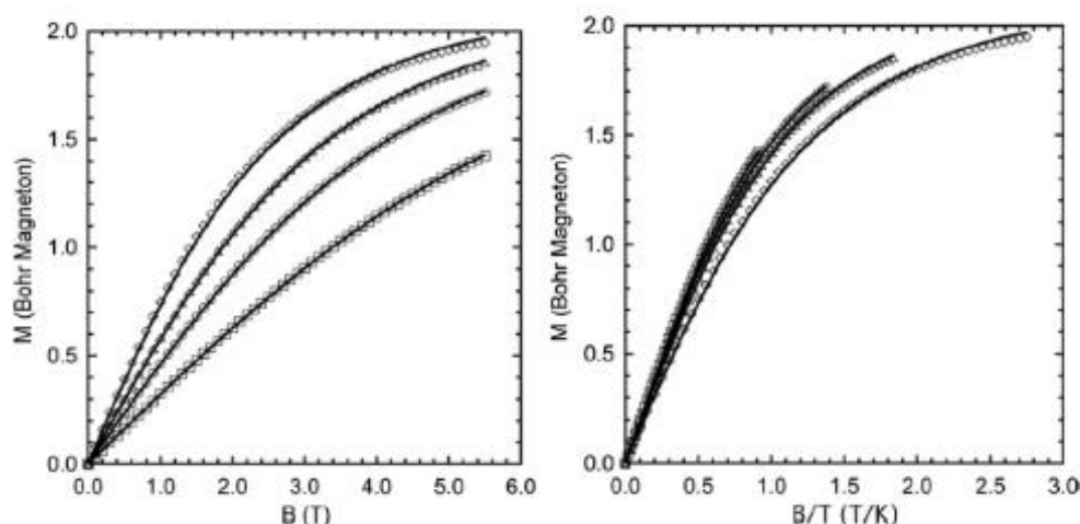
Fig. 2 Magnetization (left) and reduced magnetization (right) plots for 1 at T=2 (diamond), 3 (triangle), 4 (circle) and 6 (square) K, the lines correspond to the best fit with the positive D value (see text)
